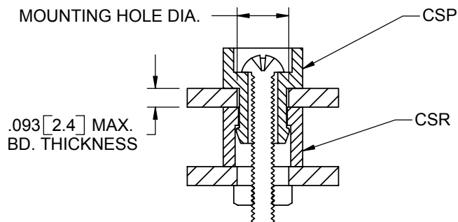
TYPICAL ASSEMBLY
